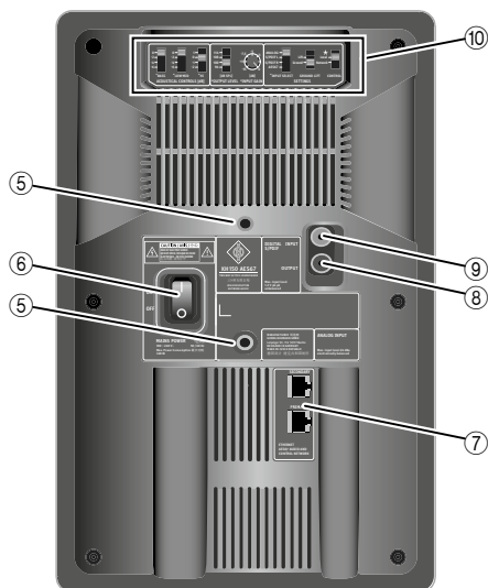
Back panel
